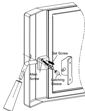
Rear View of Door shown
