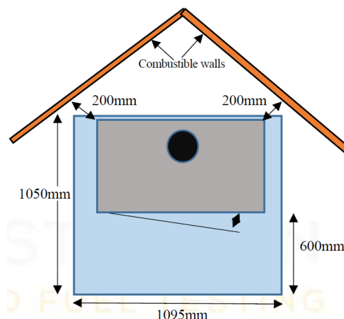
Figure No.5 - Safety distances of Loire 800 in corner position
