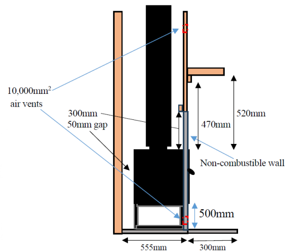
Figure No.10 - Profile view of safety distances of Loire 800 and Loire 1000 inbuilt and zero clearance box
