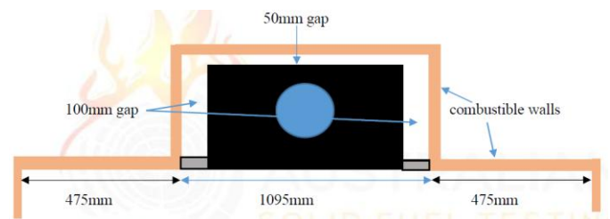
Figure No.11 - Top view of safety distances of Loire 800 inbuilt and zero clearance box
