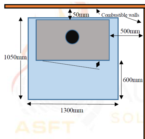
Figure No.6 - Safety distances of Loire 1000 in parallel position
