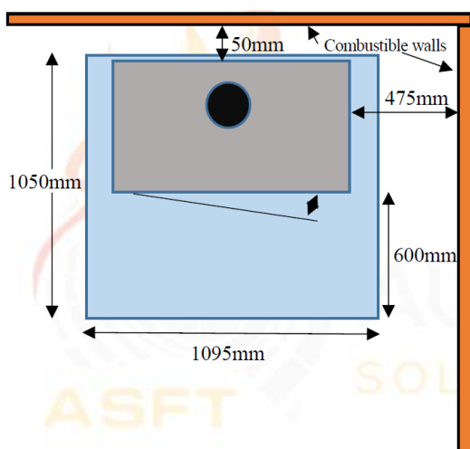
Figure No.4 - Safety distances of Loire 800 in parallel position
