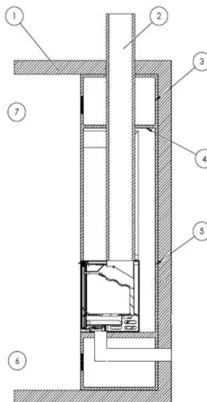
Figure No.13 - Interior diagram of the casing
