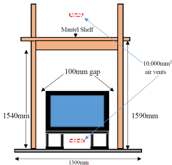
Figure No.9 - Front view of safety distances of Loire 1000 inbuilt and zero clearance box
