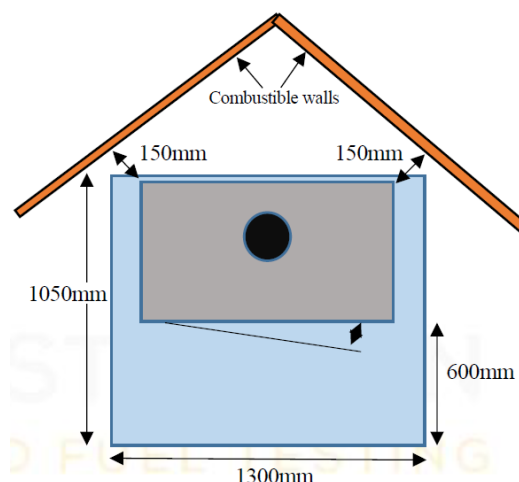
Figure No.7 - Safety distances of Loire 1000 in corner position
