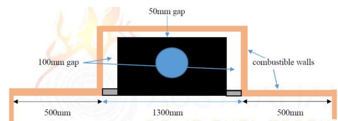
Figure No.12 - Top view of safety distances of Loire 1000 inbuilt and zero clearance box
