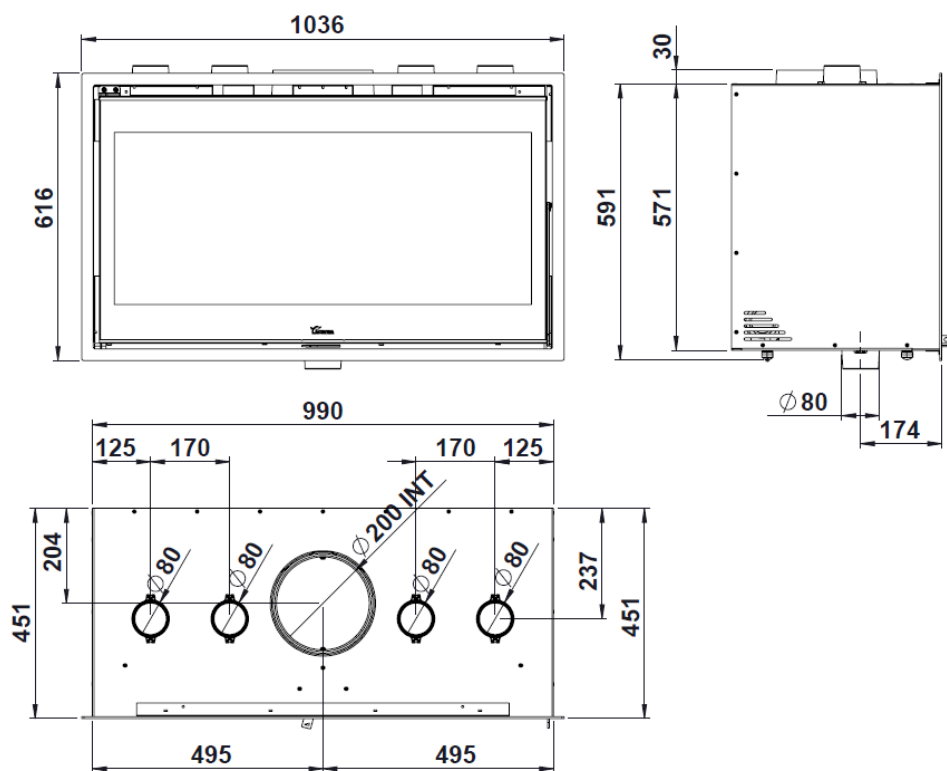
Figure No.2 - Dimensions of the LOIRE 1000 appliance in mm
