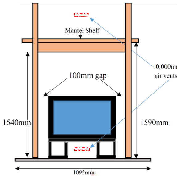
Figure No.8 - Front view of safety distances of Loire 800 inbuilt and zero clearance box
