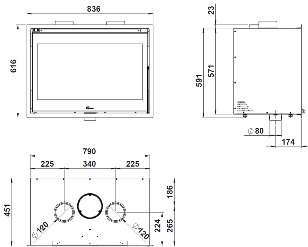
Figure No.1 - Dimensions of the LOIRE 800 appliance in mm
